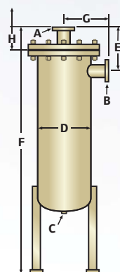
NL Module Dimensions Please refer to the table above to find dimensions for each NL model.
